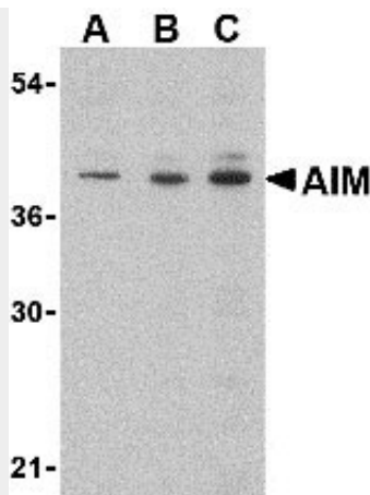
Western blot analysis of AIM in Raji lysate with AIM antibody at (A) 0.5, (B) 1 and (C) 2 \mu g/mL.
