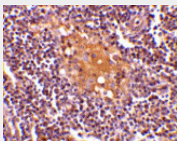
Immunohistochemistry of AIM in human lymph node tissue with AIM antibody at 10 \mu g/mL.
